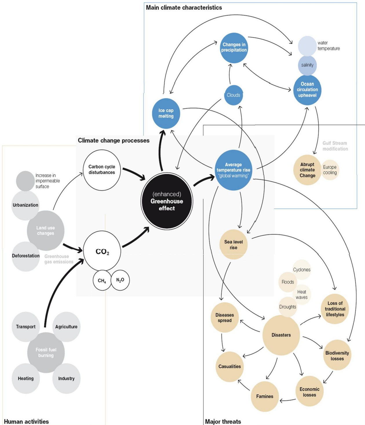
Figure 3: Climate change: processes, characteristics and threats 6
