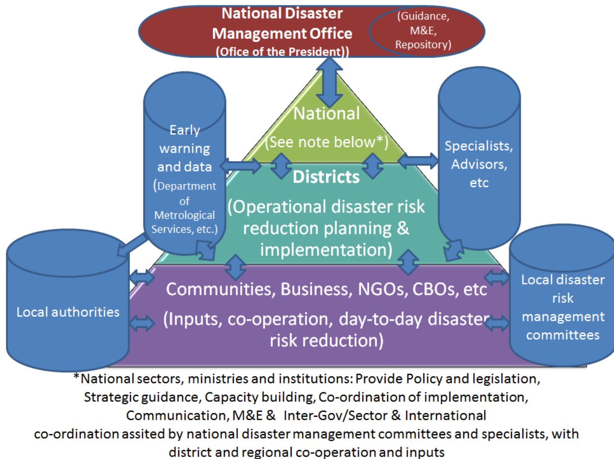
Figure 5: The first figure indicates the strategic levels where disaster risk reduction is being implemented in the country.
