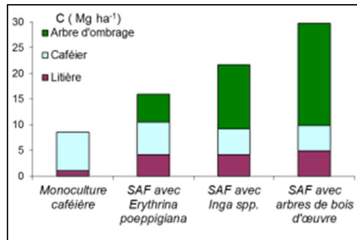
Figure 20 : Accumulation de carbone (Mg C ha -1 ) (Vaast, Harmand, Rapidel, Jagoret, & Deheuvels, 2015)
