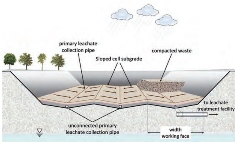
Schematic diagram of sanitary landfill with leachate system (adapted from Qian et al, 2002)
