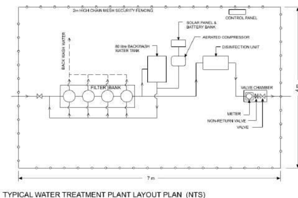
Figure 10: Concept Layout Typical Water Treatment Plant
