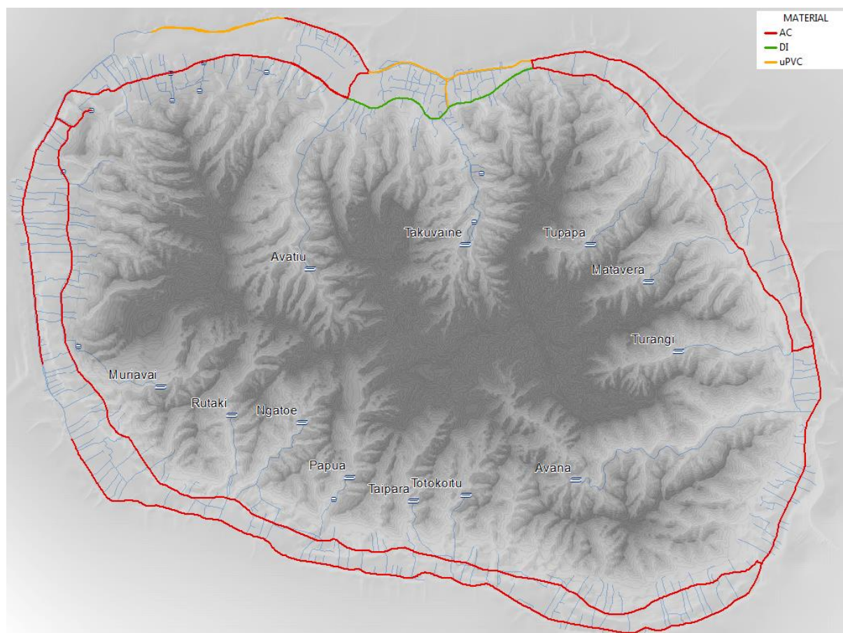
Figure 7 Ringmain pipe materials
