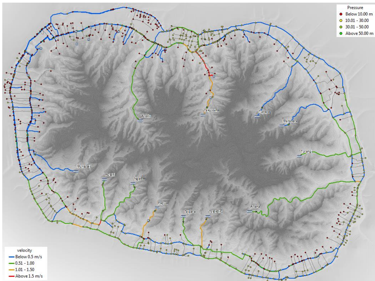
Figure 18 2016 network performance
