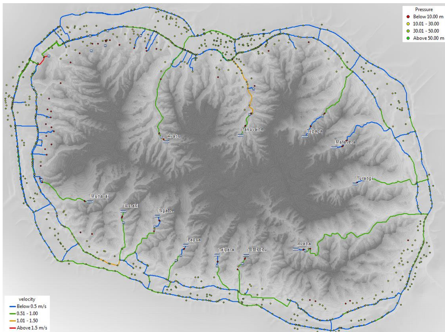
Figure 22 2031 network performance
