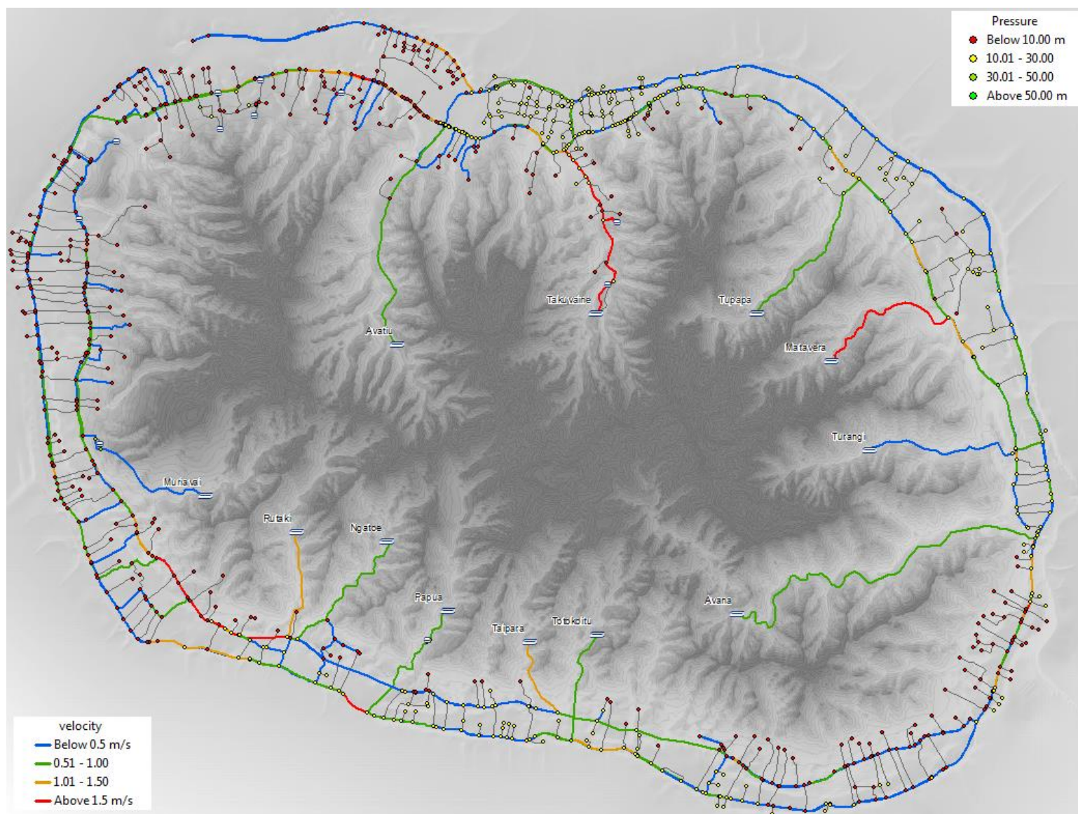
Figure 16 2013 network performance
