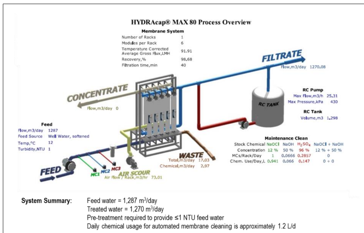
Figure 28 Hydranautics HYDRAcap MAX 80 microfiltration system
