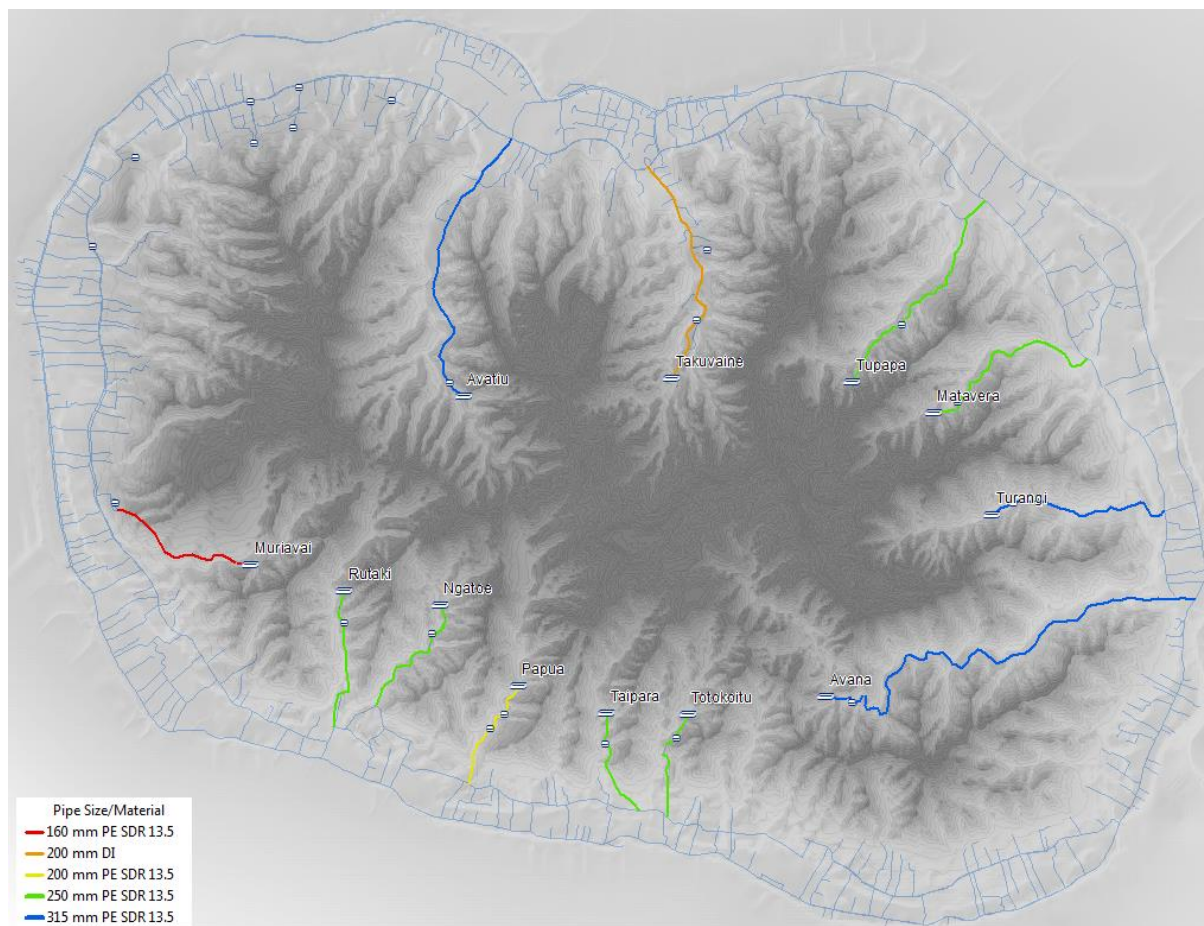
Figure 21 Rarotonga trunkmain upgrades
