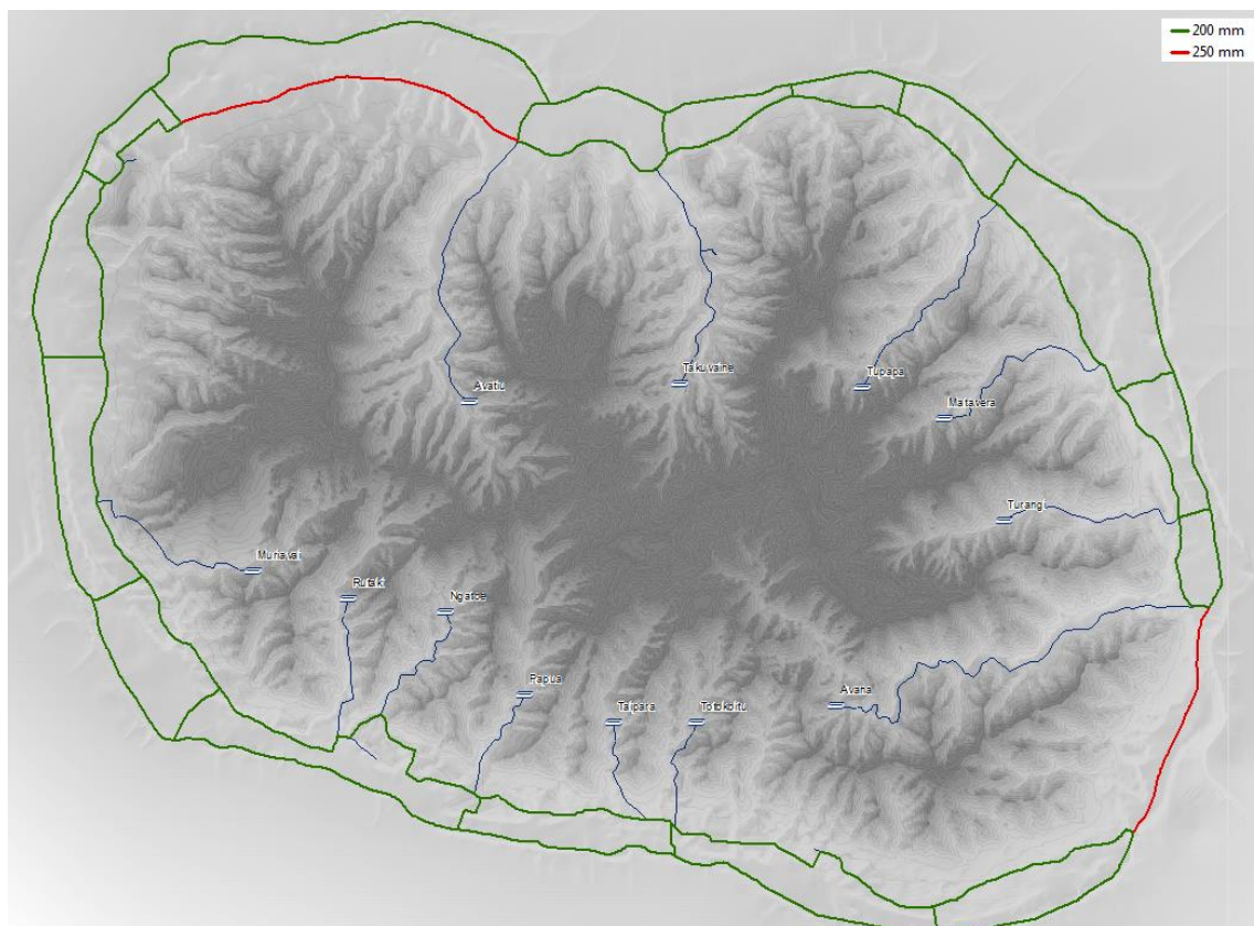
Figure 17 Proposed CCECC ringmain upgrades
