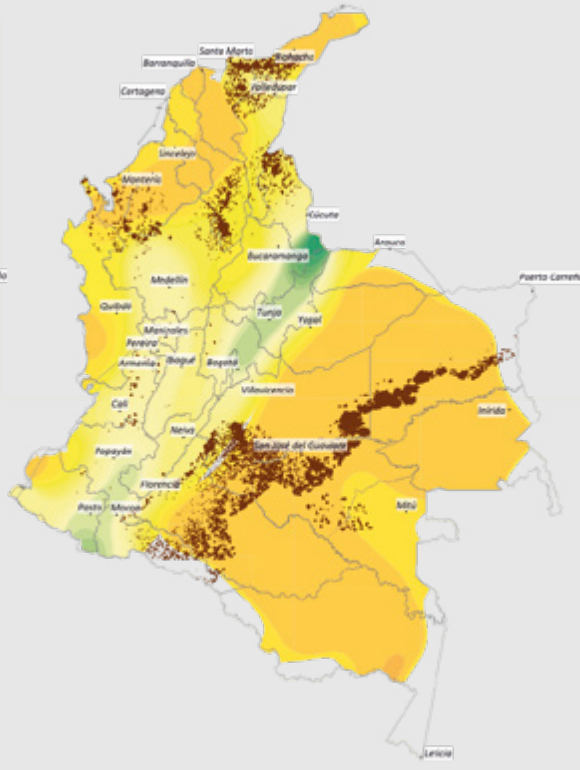
RCP IDEAM
