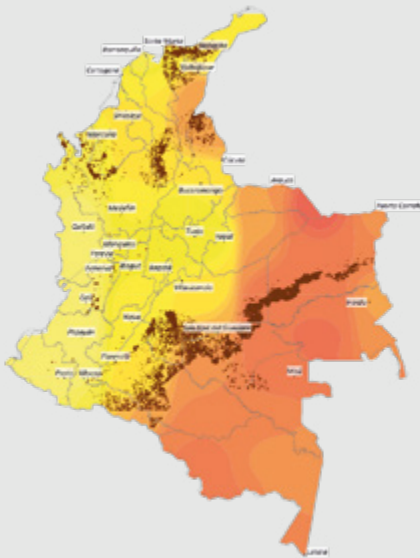
RCP 4.5
