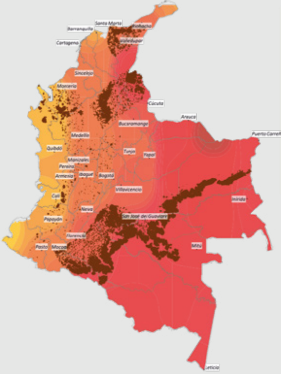
RCP 8.5
