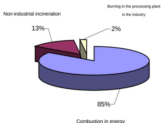
2008 PCB emissions by activity
