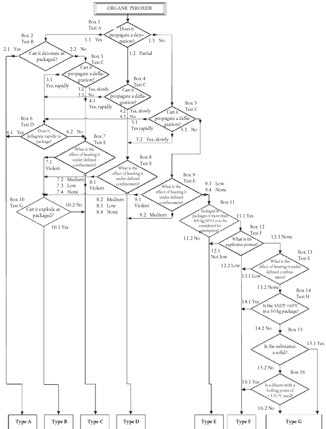
Figure 2.15.1 Organic Peroxides
