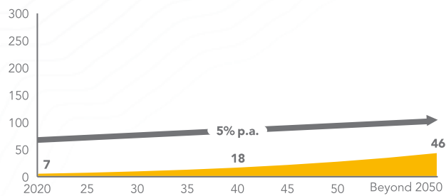
Total commercial water heating, PJ
