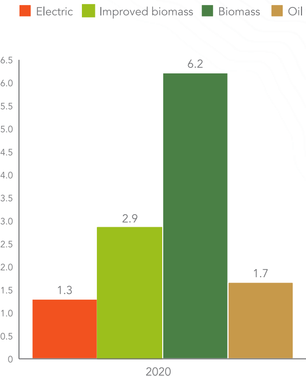
Cookstove fuel efficiency per technology, PJ of fuel / PJ of heat
