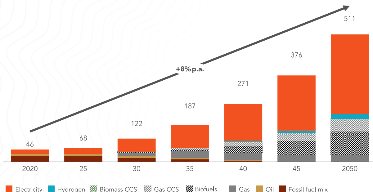
Industry Fuel Consumption, PJ
