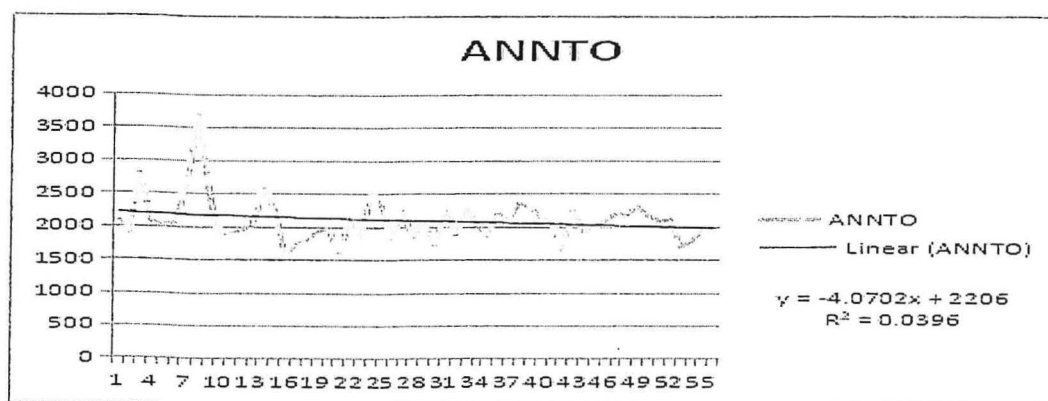
Figure 2 :Annual Rainfall
