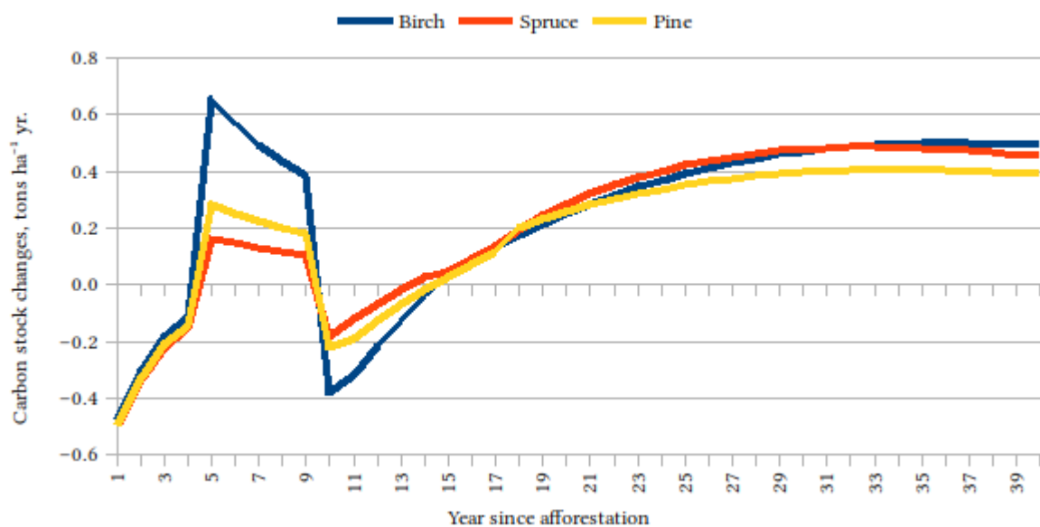
Figure 16: Projections of soil carbon stock changes in afforested lands.
