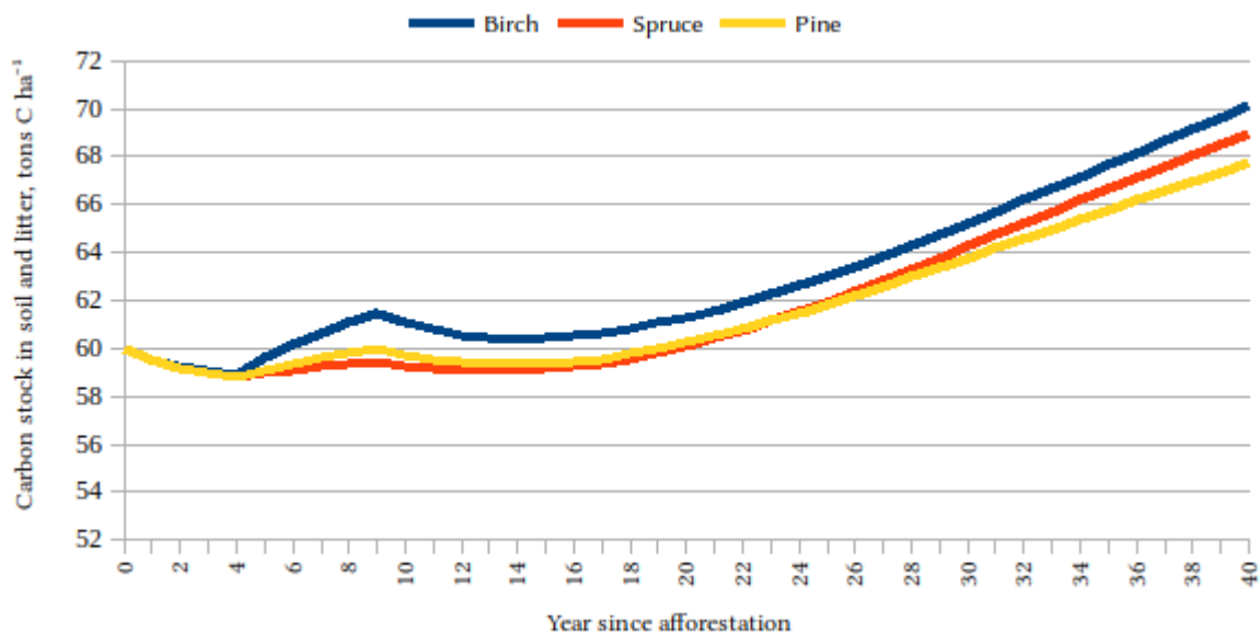
Figure 15: Projections of soil carbon stock in afforested lands.
