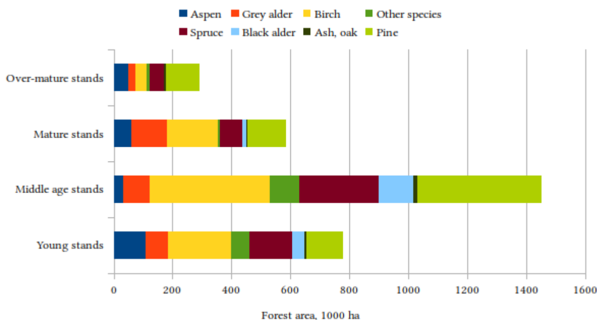
Figure 3: Forest age structure in Latvia in 2017 (NFI data).
