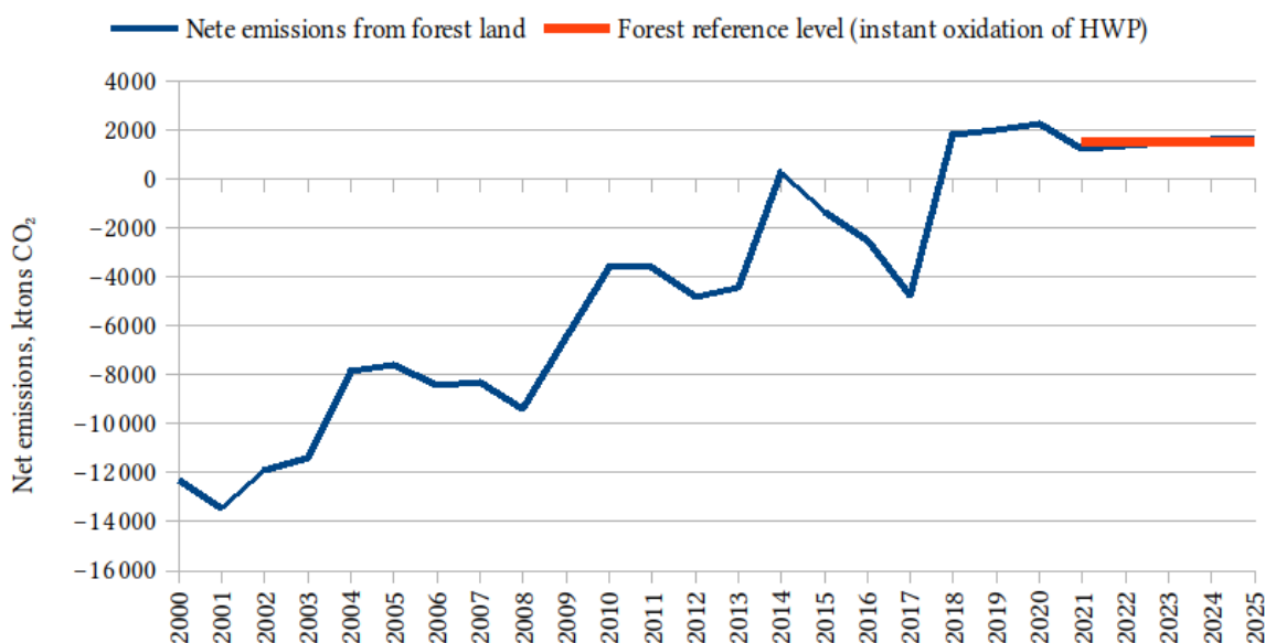
Figure 9: Forest reference level and historical GHG emissions in forest land in case of instantaneous oxidation of HWP.
