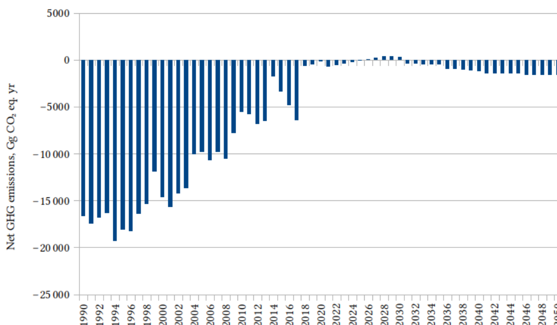
Figure 1: Net emissions in forest lands including afforestation.
