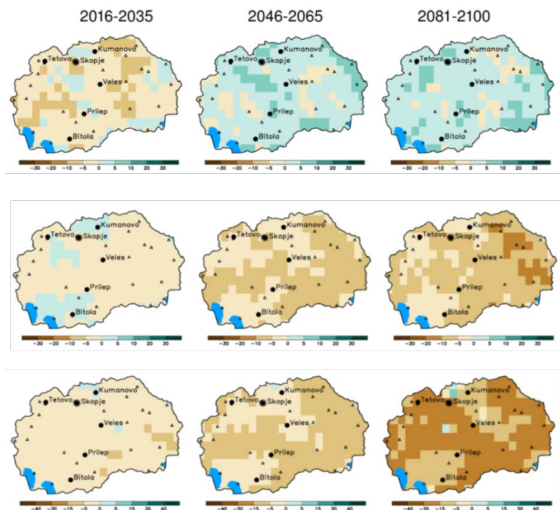
Figure 2 Future precipitation change, for three future periods, 2016-2035, 2046-2065 and 2081-2100 with respect to the period 1986-2005 for the low, mid and high scenarios (top, middle and bottom respectively).*
