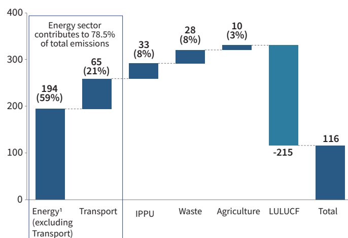
Malaysia's GHG inventory, MtCO 2 eq (2019) from BUR4
