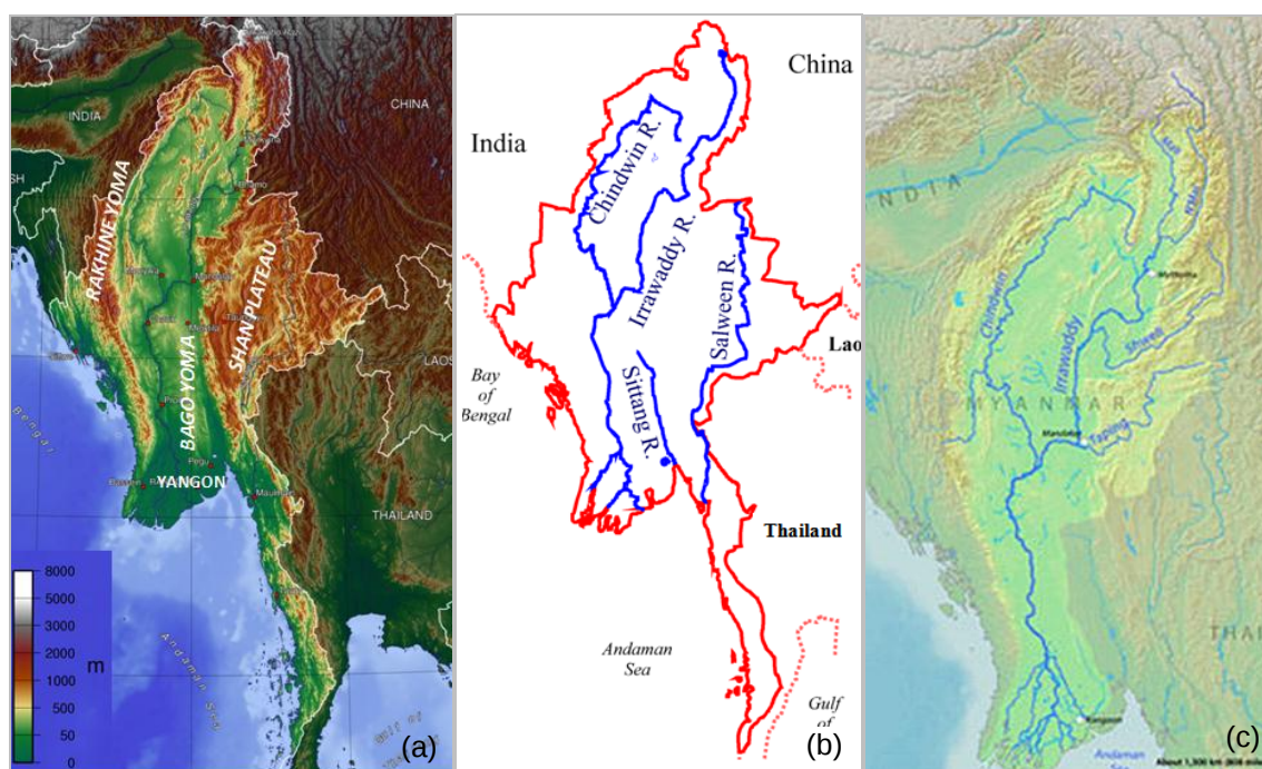
Figure 3. (a) Elevation above sea-level and mountain ranges in Myanmar 18 ; (b) major rivers in Myanmar and (c) the Ayeyarwaddy River Basin 19 .
