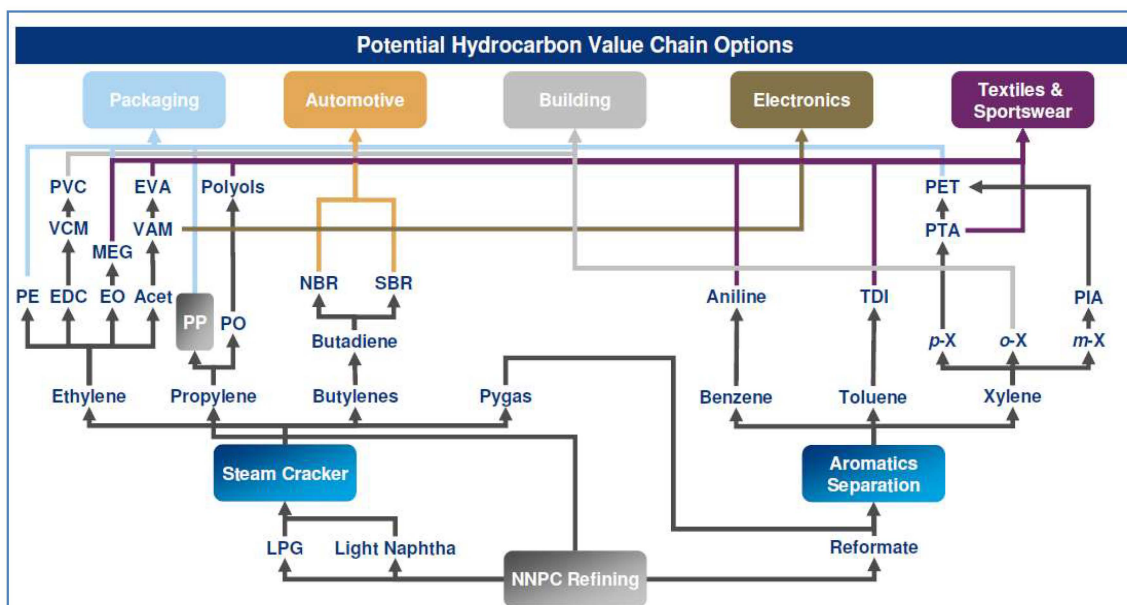
Figure 24: Options for Petrochemicals from the Hydrocarbon Value Chain
