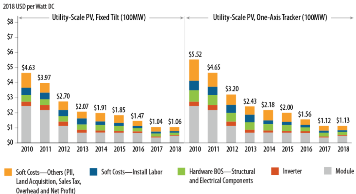
Figure 3. PV Solar Cost Trends
