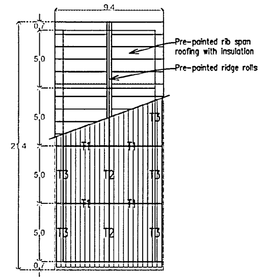
ROOF PLAN
