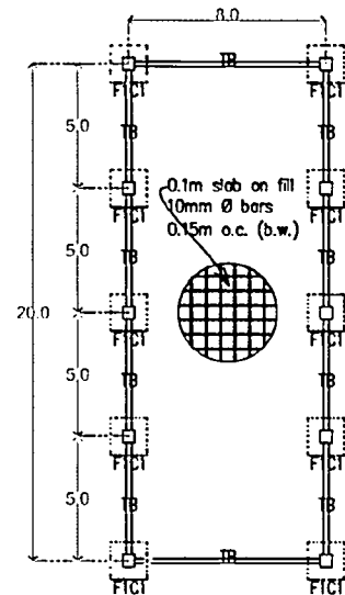
FOUNDATION PLAN
