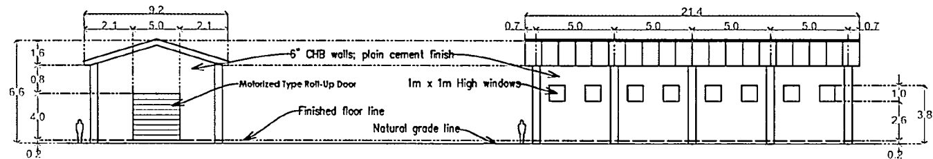
FRONT ELEVATION
