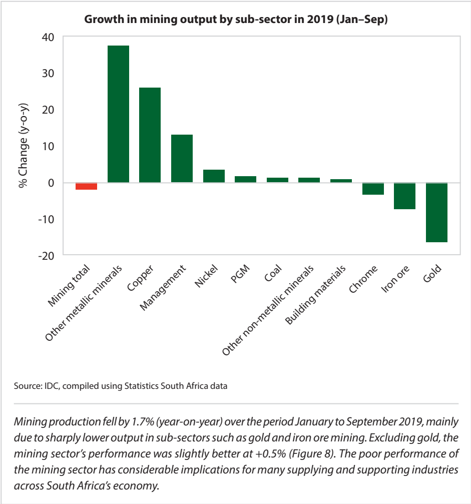
Figure 8: Mining output
