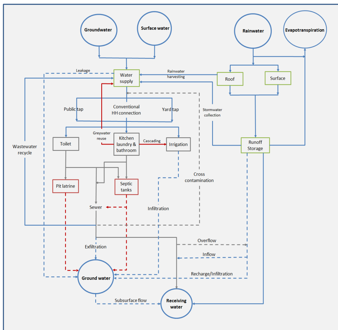
Figure 11. A tailored integrated urban water infrastructure for cities in sub-Saharan Africa 66
