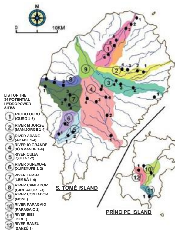
Figure 13: Sites with hydropower potential in STP (ALER/STP Government, 2019)
