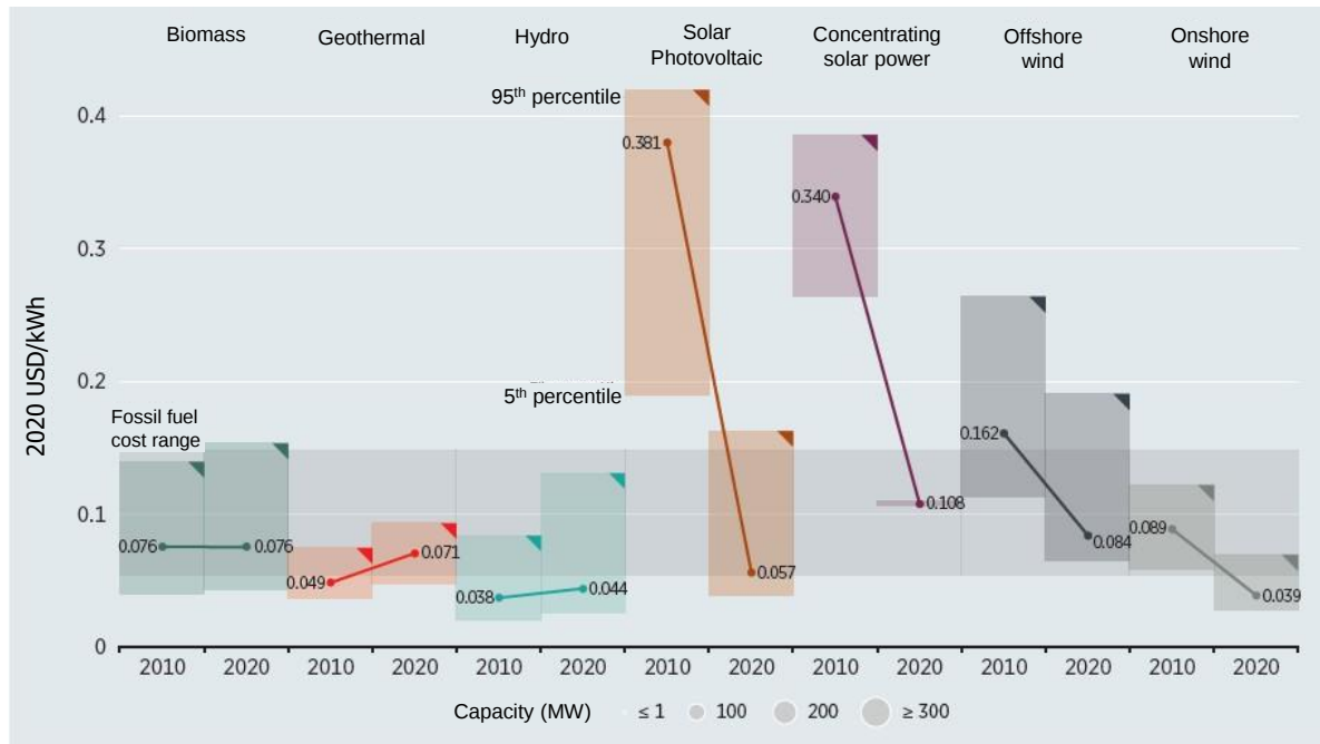
Figure 18: Global LCOE of different newly installed renewable generation plants, 2010-2020 (IRENA, 2021)
