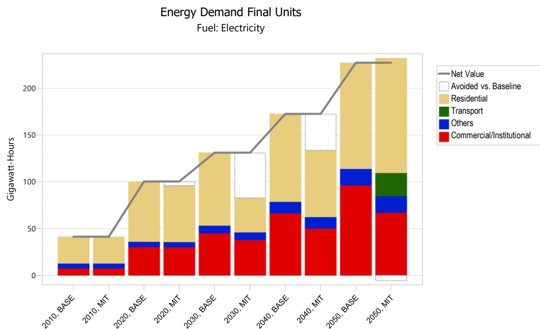
Figure 27: Comparison of baseline and mitigation scenarios on electricity demand by sector (in GWh), in 10-year periods
