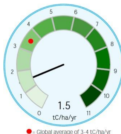
● = Global average of 3-4 tC/ha/yr Figure 12: Biomass potential in terms of Net Primary Production (IRENA, 2017)
