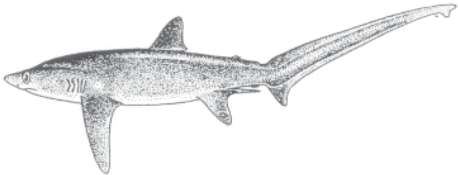
Alopius superciliosus
