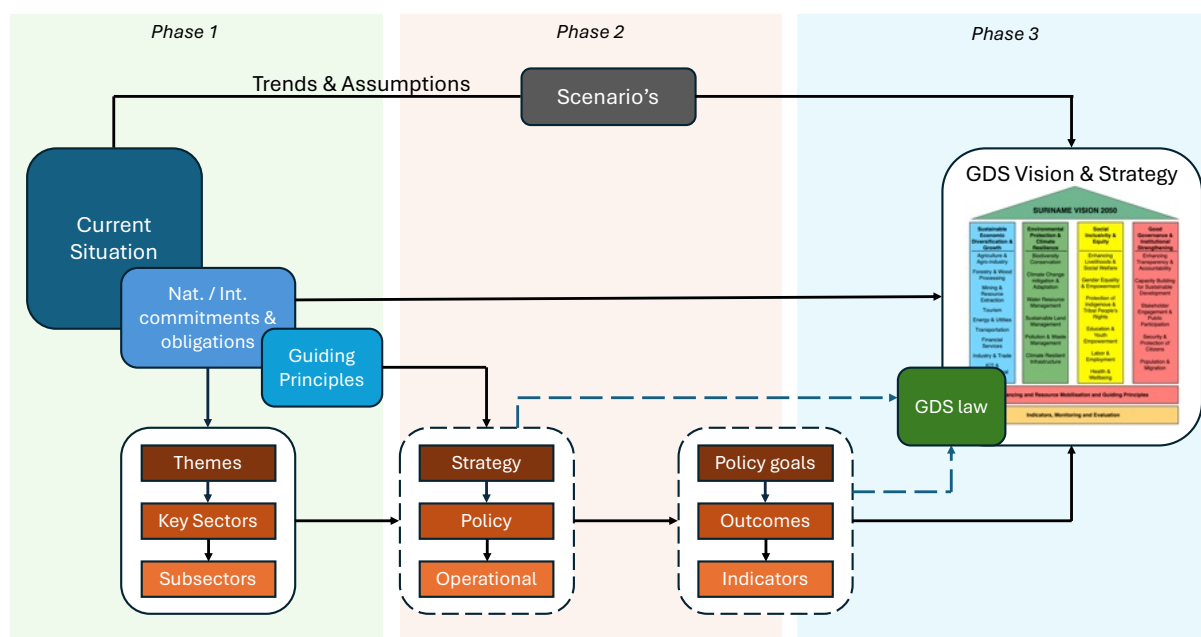
Figure 12: GDS Methodology
