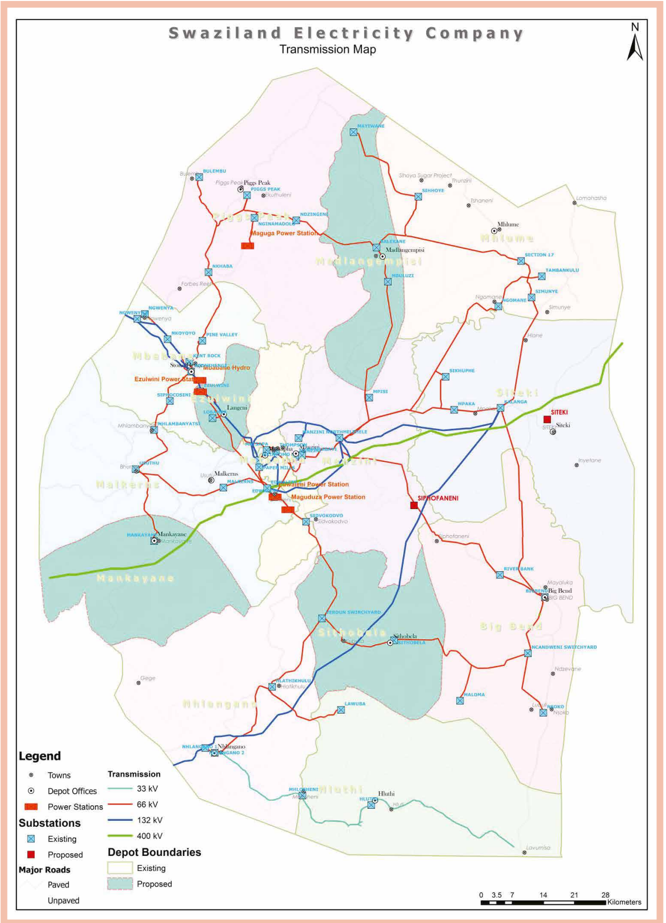
FIGURE 7.4 TRANSMISSION SYSTEM MAP
