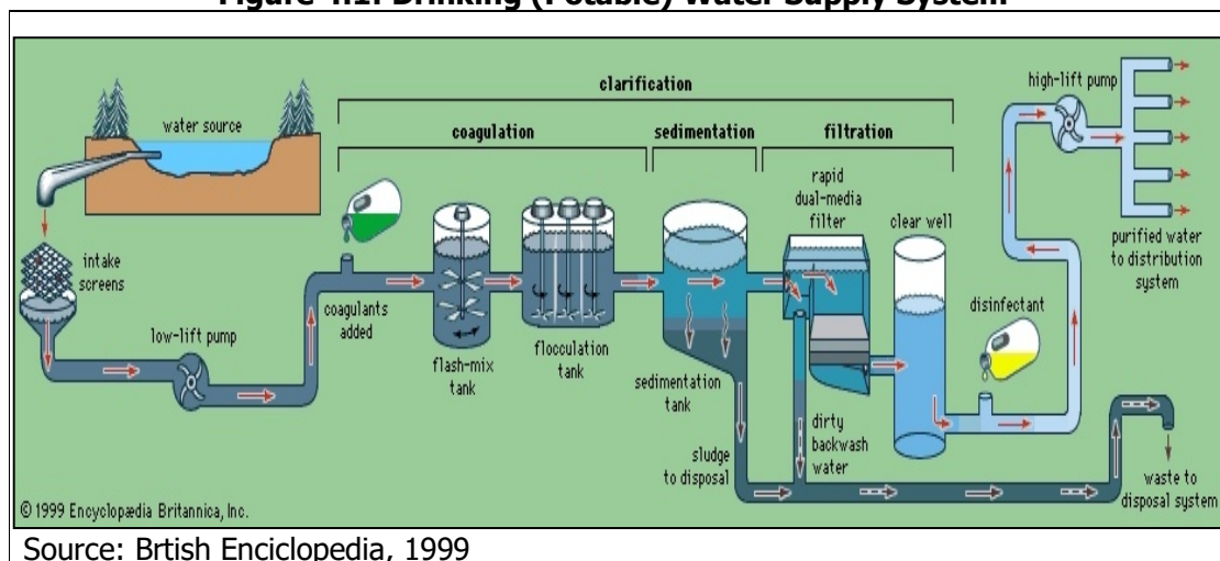
Figure 4.1: Drinking (Potable) Water Supply System
