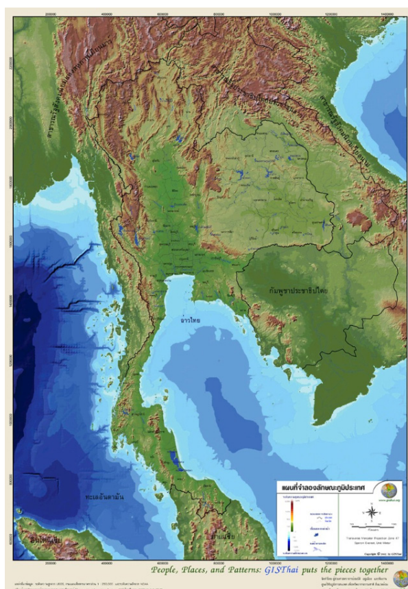
Figure 1-1: Thailand's topographic map.
