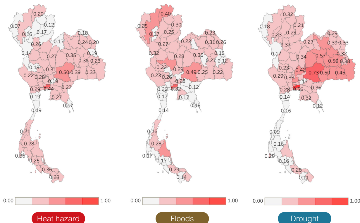
Figure 3-7: Risk areas for the human settlements and security sector under the RCP4.5 with a focus on heat hazard, floods, and drought areas shown in the country map during 2016-2035. The darker color indicates more severely impacted areas.
