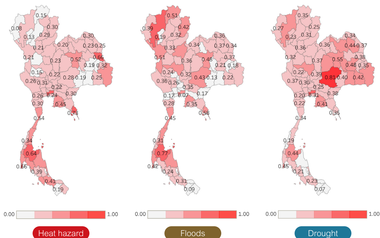
Figure 3-4: Risk areas for the tourism sector under the RCP4.5 with the focus on heat hazard, floods, and drought areas shown in the country map during 2016-2035. The darker color indicates more severely impacted areas.
