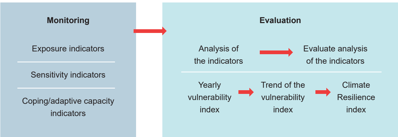
Figure 5-2: Framework to monitor and evaluate Thailand’s resilience.
