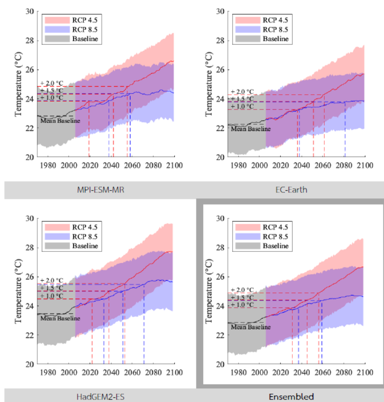
Figure 1-5: Future changes in temperature in Thailand.
