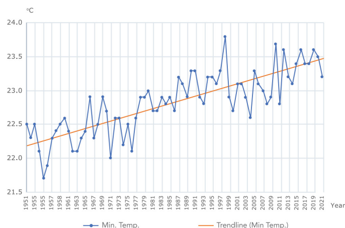
Figure 1-4: Annual mean minimum temperature in Thailand (°C) during 1951-2021.
