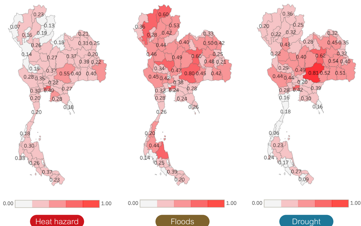
Figure 3-2: Risk areas for the water resources management sector under RCP4.5 with a focus on heat hazard, floods, and drought area shown in the country map during 2016-2035. The darker color indicates more severely impacted areas.
