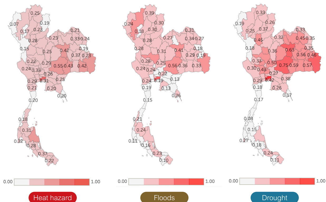
Figure 3-5: Risk areas for the public health sector under the RCP4.5 with a focus on Heat hazard, floods, and drought areas shown in the country map during 2016-2035.
