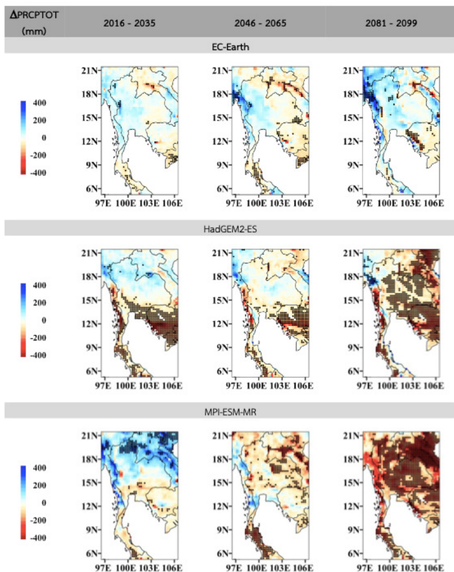
Figure 1-8: Projection of the PRCPTOT anomaly under RCP4.5.
