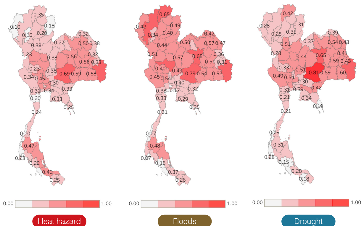
Figure 3-3: Risk areas for the agriculture and food security sector under RCP4.5 with a focus on heat hazard, floods, and drought areas shown in the country map during 2016-2035. The darker color indicates more severely impacted areas.
