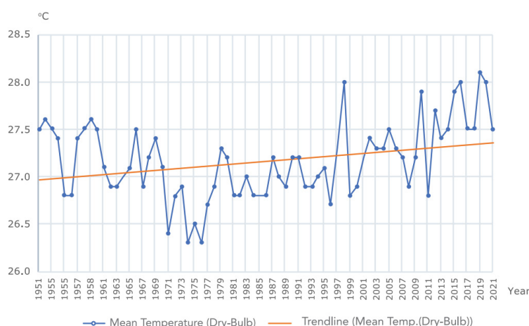
Figure 1-2: Annual mean temperature (dry-bulb) in Thailand ( ^{\circ}\text{C} ) during 1951-2021.
