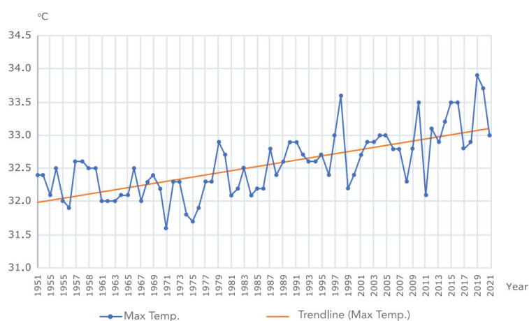
Figure 1-3: Annual mean maximum temperature in Thailand ( ^{\circ}\text{C} ) during 1951-2021.
