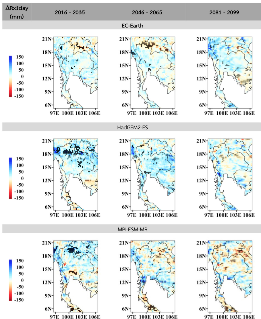
Figure 1-7: Projection of an Rx1day anomaly under RCP4.5.
