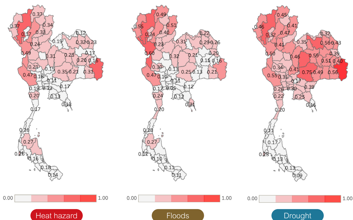
Figure 3-6: Risk areas for the natural resources sector under the RCP4.5 with a focus on Heat hazard, floods, and drought areas shown in the country map during 2016-2035. The darker color indicates more severely impacted areas.
