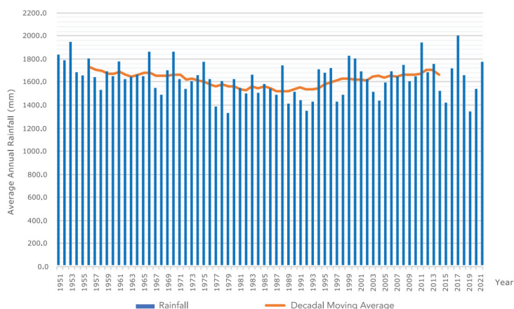
Figure 1-6: Annual mean rainfall in Thailand (mm) during 1951-2021.
