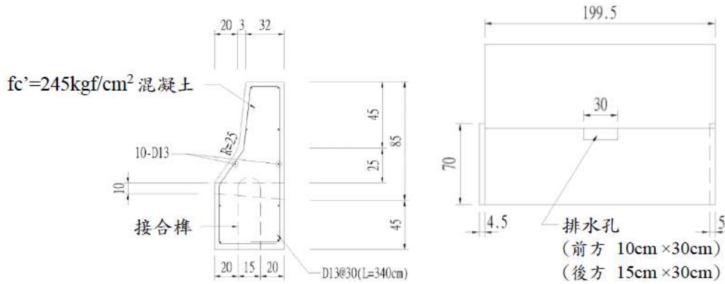
斷面及配筋
