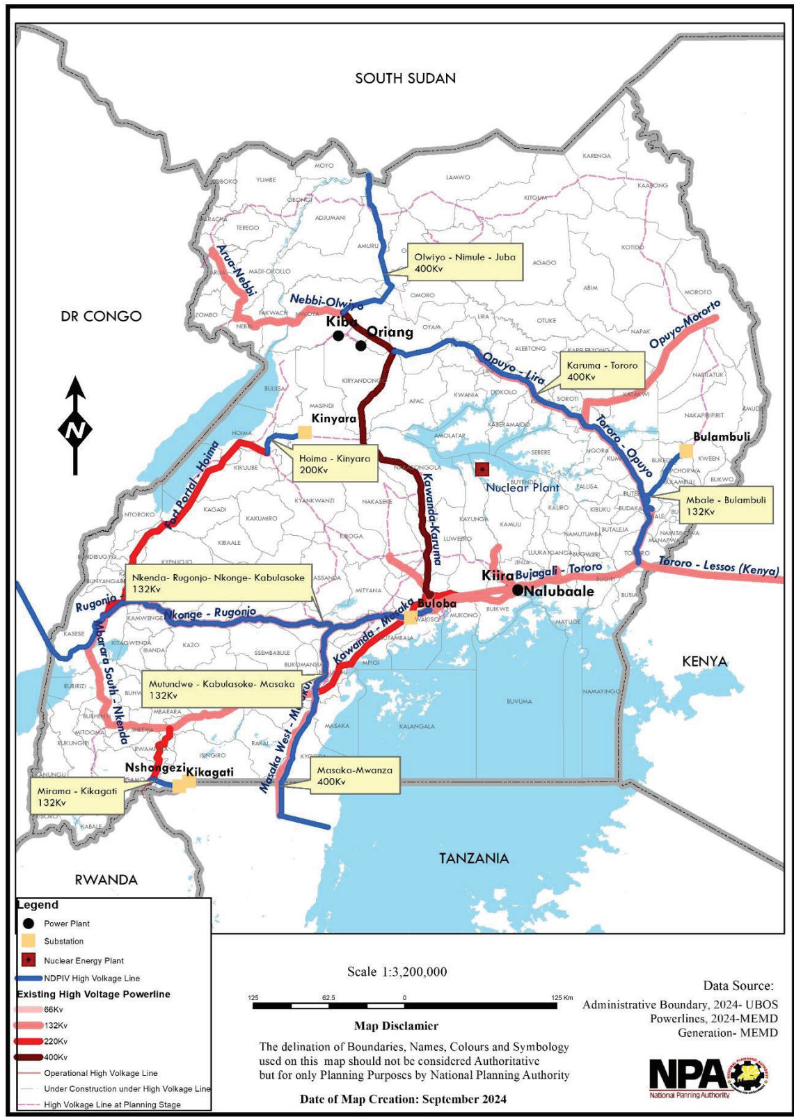
Figure 14.1: Mapping of existing powerlines and power projects to be implemented under the NDPIV
