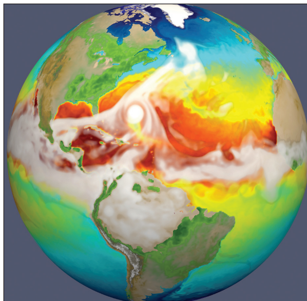
Fig. 10. Sea Surface Temperature Change. The high-resolution Energy Exascale Earth System Model (E3SM) simulates the strongest storms with surface winds exceeding 150 miles per hour, such as hurricanes that leave cold wakes 2–4 °C cooler than their surrounding waters. This simulation represents how sea surface temperature changes evolve as a hurricane (seen here approaching the U.S. East Coast) moves across the Atlantic and how the resultant cold wake affects subsequent intensification of the next hurricane. [Courtesy Los Alamos National Laboratory]
