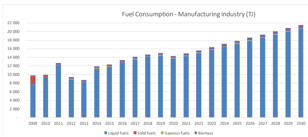
Figure 30. Fuel consumption – manufacturing industry (BAU)
