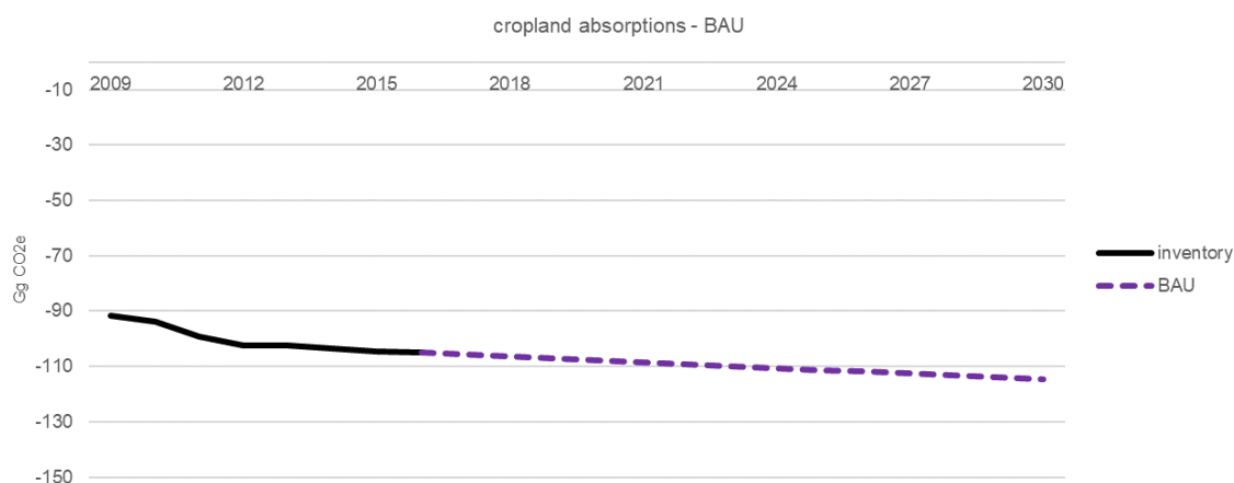
Figure 60. Projected CO 2 absorptions for cropland
