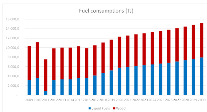
Figure 37. Fuel consumption – residential (BAU)
