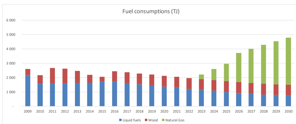
Figure 36. Fuel consumption – commercial (NDC)
