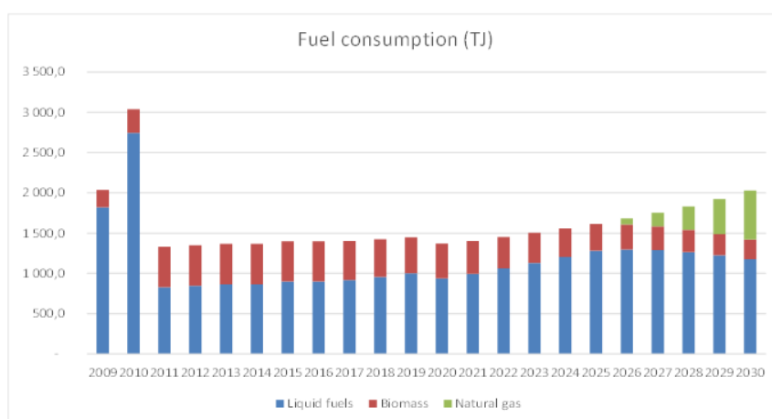
Figure 40. Fuel consumption – agriculture (NDC)
