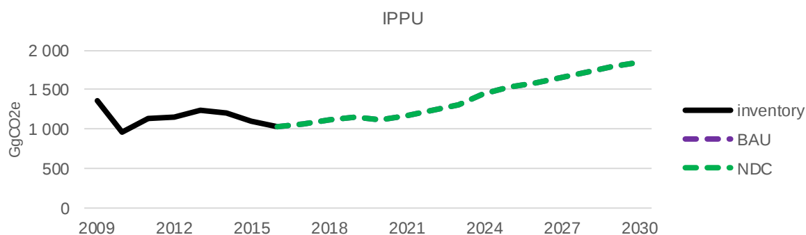
Figure 16. Projections for IPPU sector
