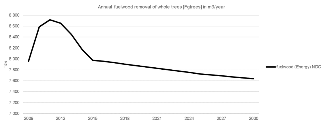
Figure 61. Projected fuelwood harvest for the NDC scenario
