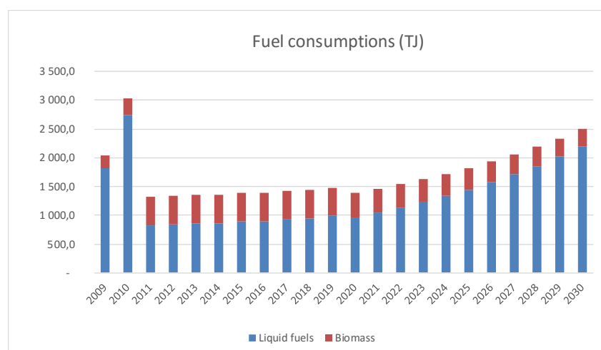
Figure 39. Fuel consumption – agriculture (BAU)
