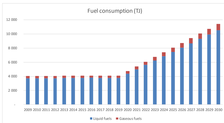
Figure 29. Fuel consumption – petroleum refining (BAU; NDC)
