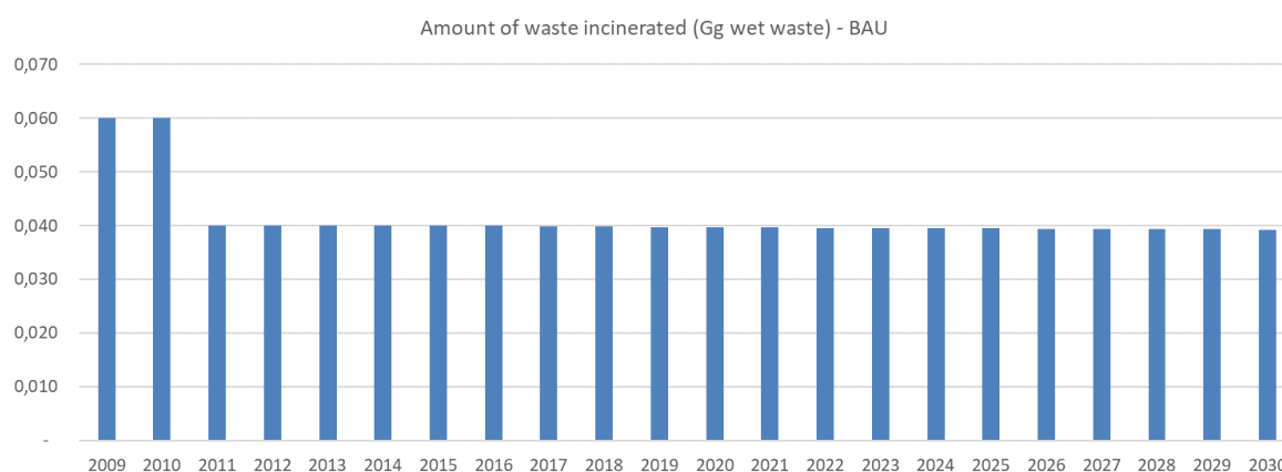
Figure 46. amount of waste incinerated - NDC
