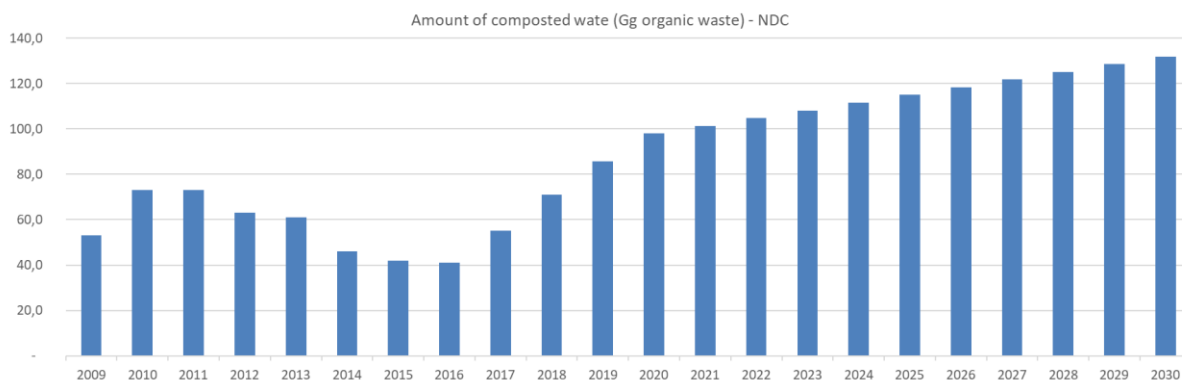
Figure 44. amount of composted waste - NDC
