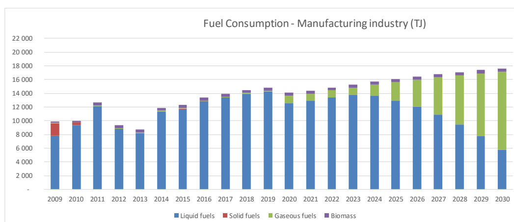
Figure 31. Fuel consumption – manufacturing industry (NDC)
