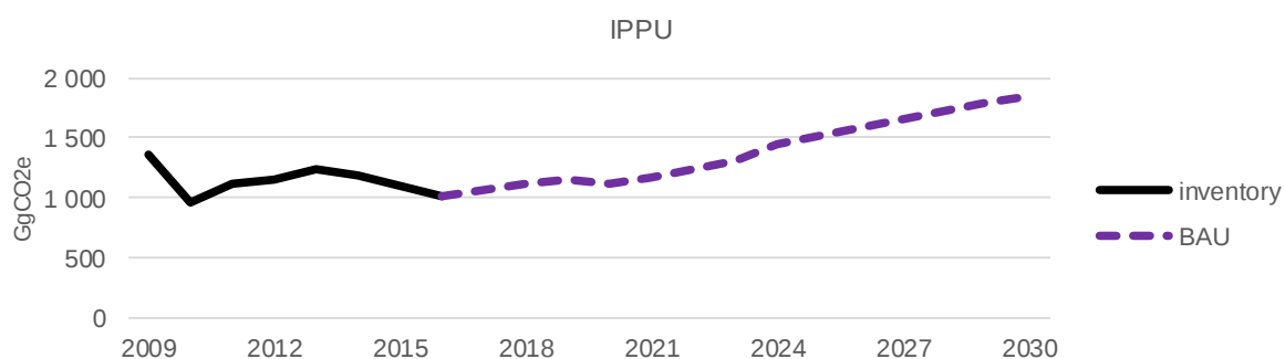
Figure 15. Projected IPPU-related emissions
