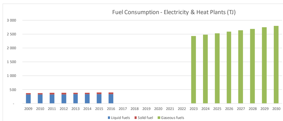
Figure 28. Fuel consumption – electricity and heat plants (NDC)
