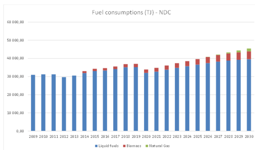
Figure 34. Fuel consumption – road transport (NDC)
