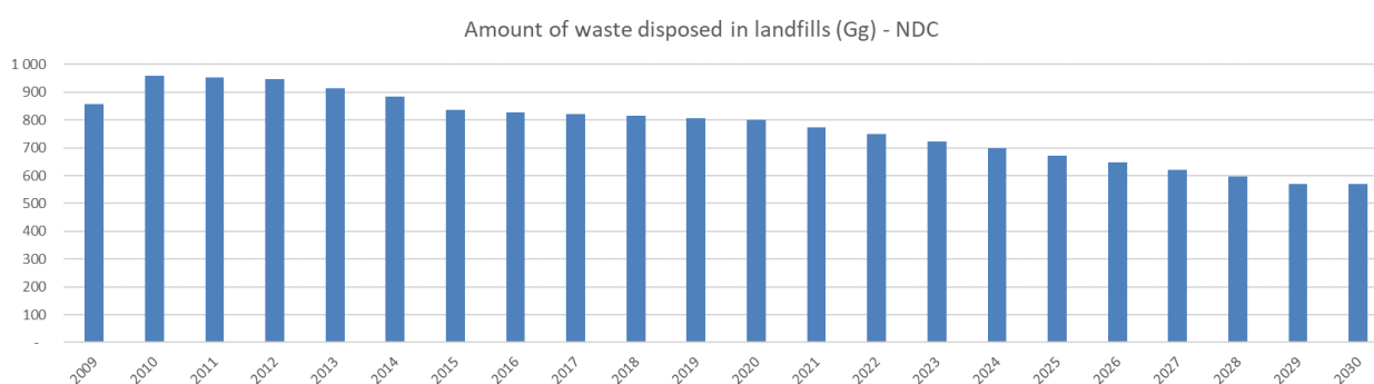
Figure 42. amount of waste disposed in landfills - NDC
