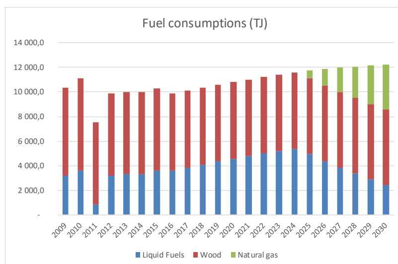
Figure 38. Fuel consumption – residential (NDC)
