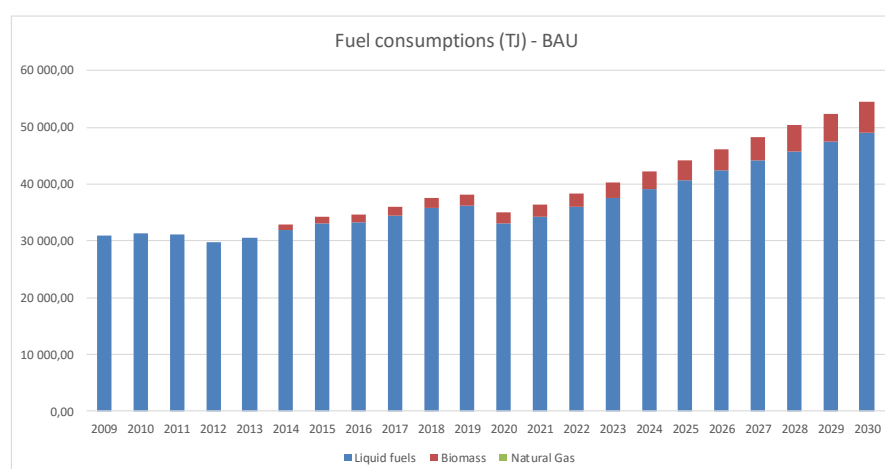
Figure 33. Fuel consumption – road transport (BAU)
