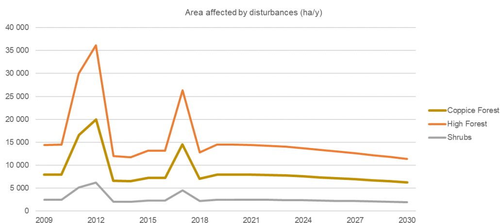
Figure 62. projected forest disturbances for the NDC scenario
