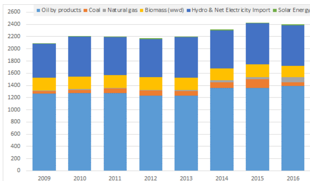
Figure 10. Energy supply (ktoe) by energy source for the period 2009-2016
