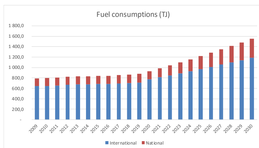
Figure 32. Fuel consumption – domestic and international aviation (BAU; NDC)
