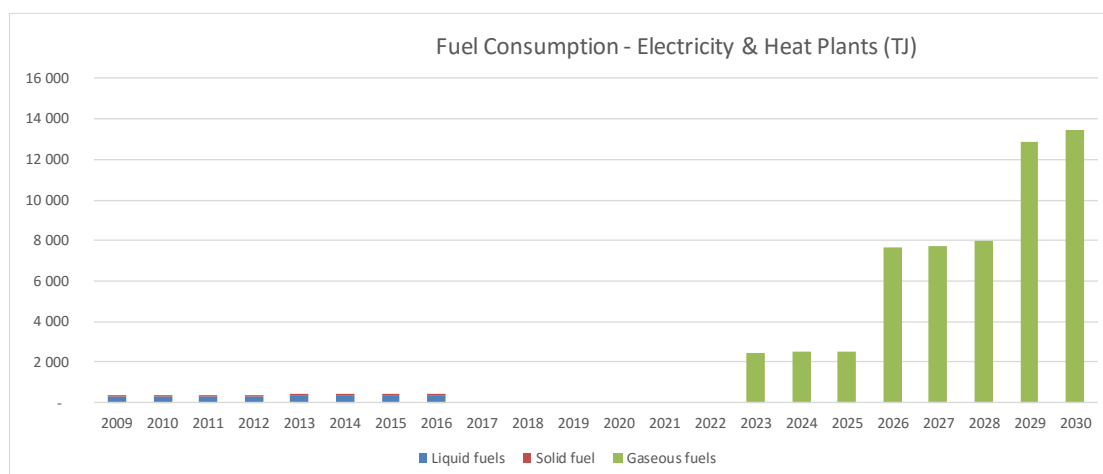
Figure 27. Fuel consumption – electricity and heat plants (BAU)
