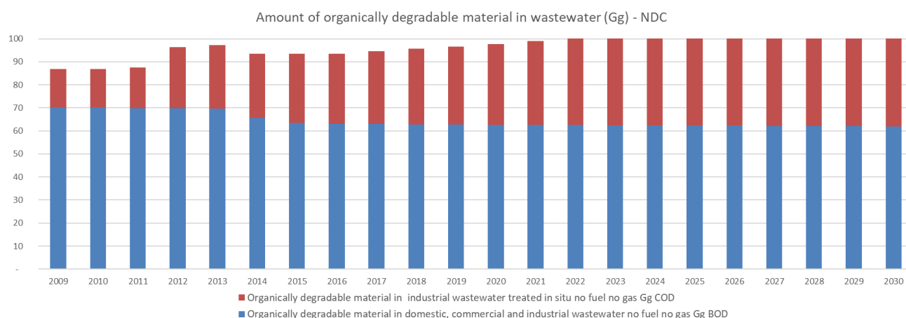
Figure 50. amount of organically degradable material in wastewater - NDC
