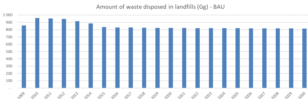
Figure 41. amount of waste disposed in landfills - BAU
