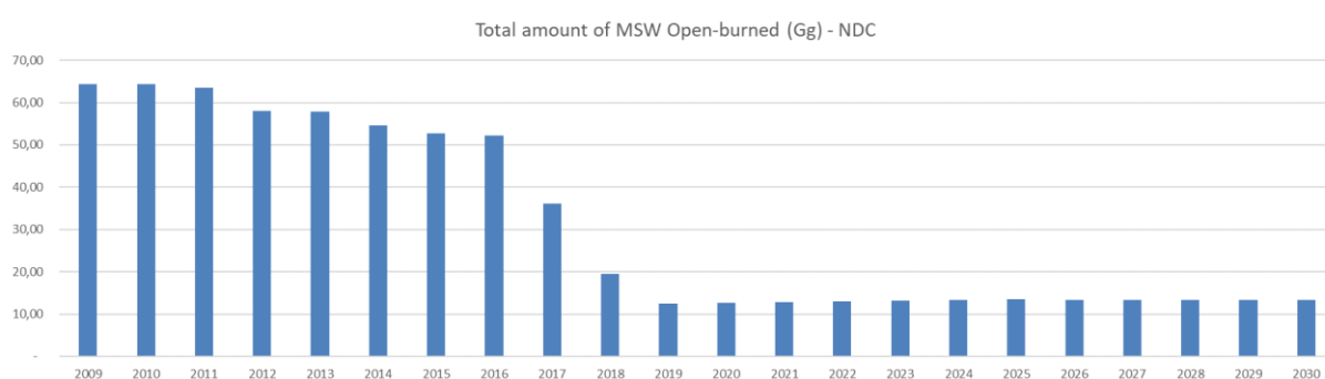
Figure 48. amount of municipal solid waste (MSW) open-burned - NDC
