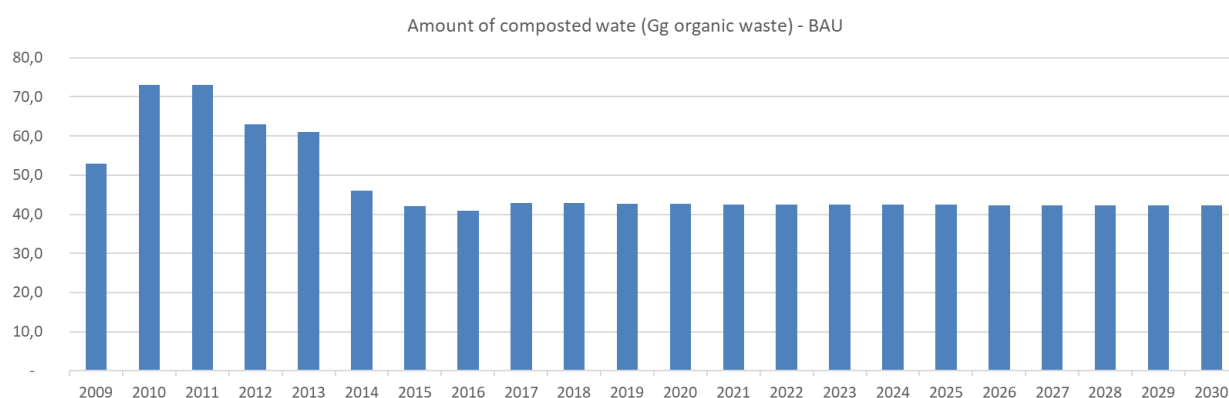
Figure 43. amount of composted waste - BAU
