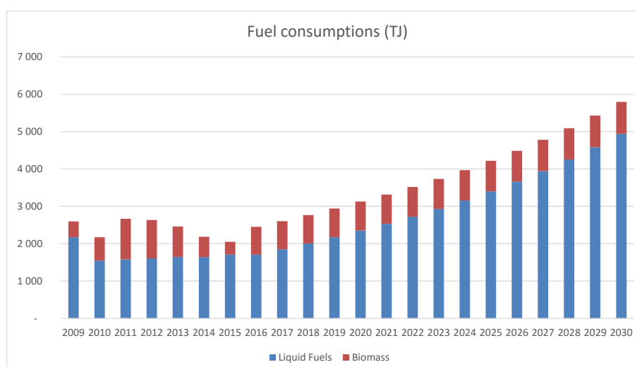
Figure 35. Fuel consumption – commercial (BAU)
