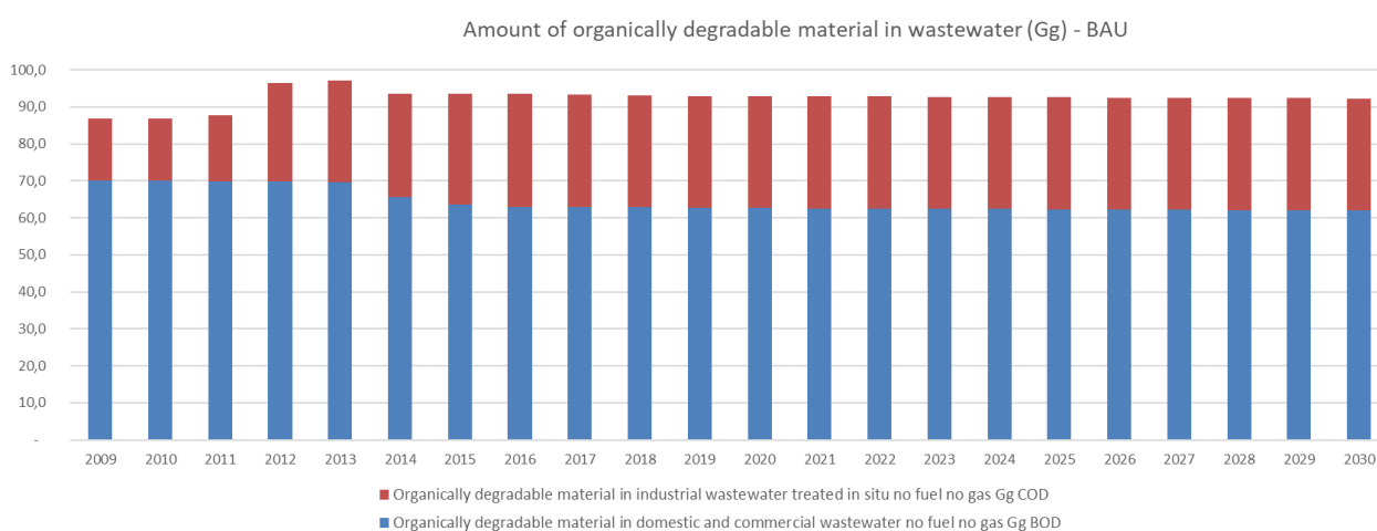
Figure 49. amount of organically degradable material in wastewater - BAU
