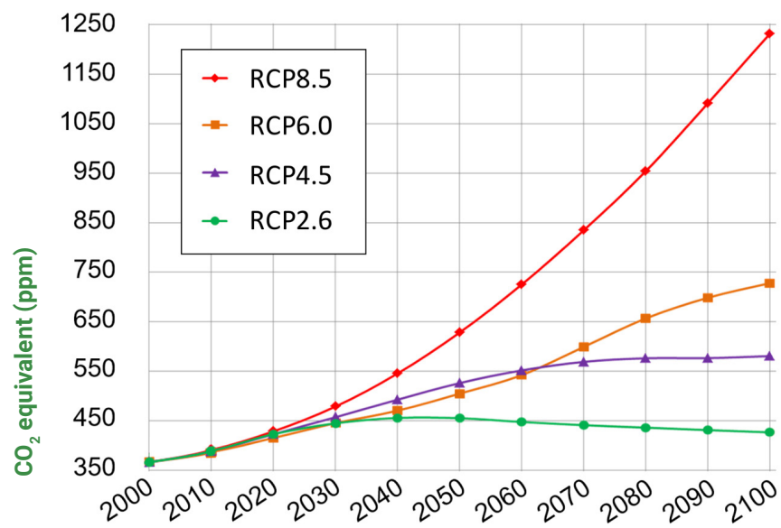
Figure 2. Future GHG concentrations for four different scenarios
