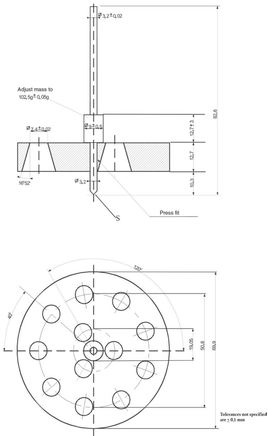
Figur 1 – Penetrometer
