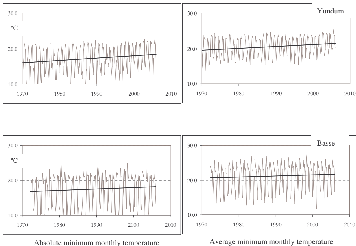
Figure 1.5: Trends in minimum temperature at Yundum and Basse, showing respectively increases of 0.67 and 0.40 degree Celsius per decade in the average minimum monthly temperatures. Line slopes (i.e. rate of change) verified as statistically significant at the 95% confidence level.
