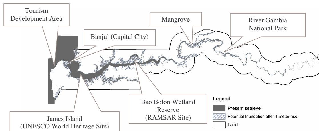
Figure 2.1: Area liable to permanent flooding from a 100 cm sea level rise scenario. Notice that total area flooded also depends on diurnal tidal cycles and seasonal flooding. Erosion of beaches and potential breaching of barrier dunes on the Atlantic seaboard, as a result of increased wave activity could further aggravate the degree of flooding in coastal areas. Map and statistics prepared by Dr. Malanding S. Jaiteh using Gambia 50000 GIS Database 2003 and ArcGIS Spatial Analysis Extension
