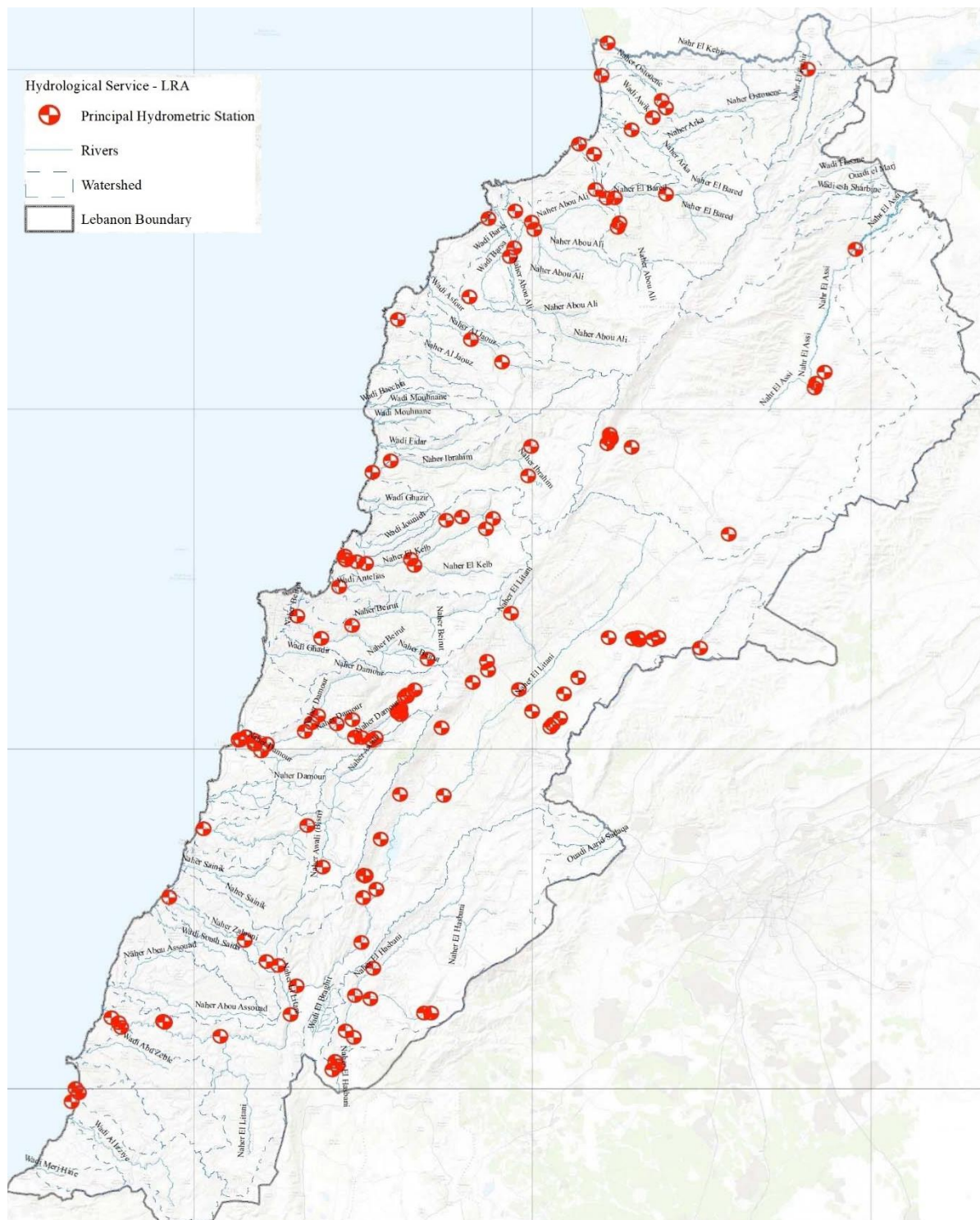
Figure III B 20 Hydrometric stations of the Lebanese Hydrological Service at the LRA in 2016
