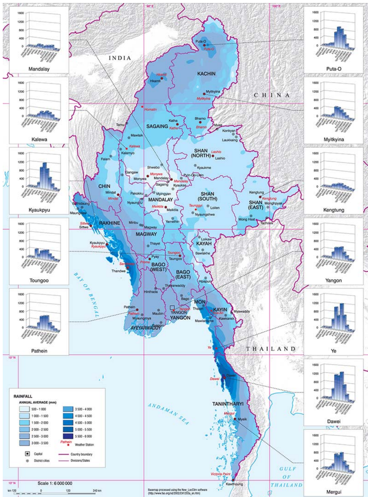
Figure 4-4 Detailed rainfall map with selected monitoring stations [FAO, 2002]
