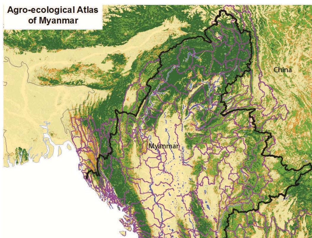
Figure A 4 Agro-ecological Atlas of Myanmar [source Earl Saxon, Forest Inform]
