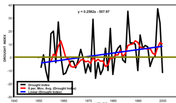
Figure 5-5 Droughts in Myanmar
