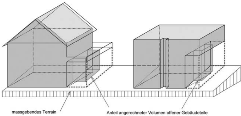
Figur 8.3 Baumassenziffer
