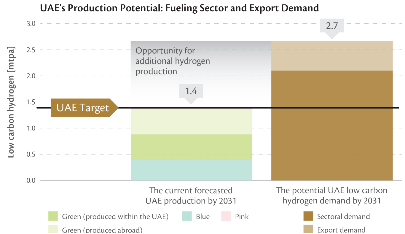
Figure 2 The UAE's 2031 production potential
