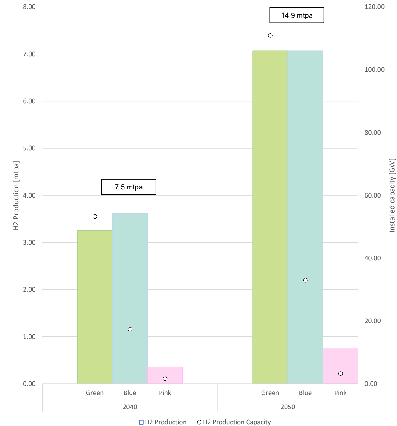
Figure 7 Forecasted UAE production requirement including low export potential. Source: Fraunhofer CINES.
