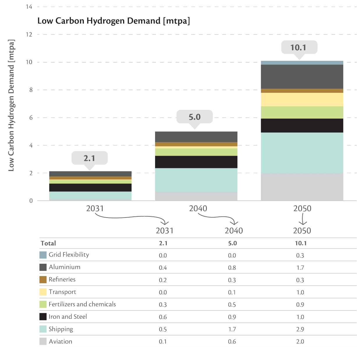
Figure 4 UAE Low Carbon Hydrogen Sectoral Demand from 2031 to 2050 in mtpa. Source: Fraunhofer CINES.
