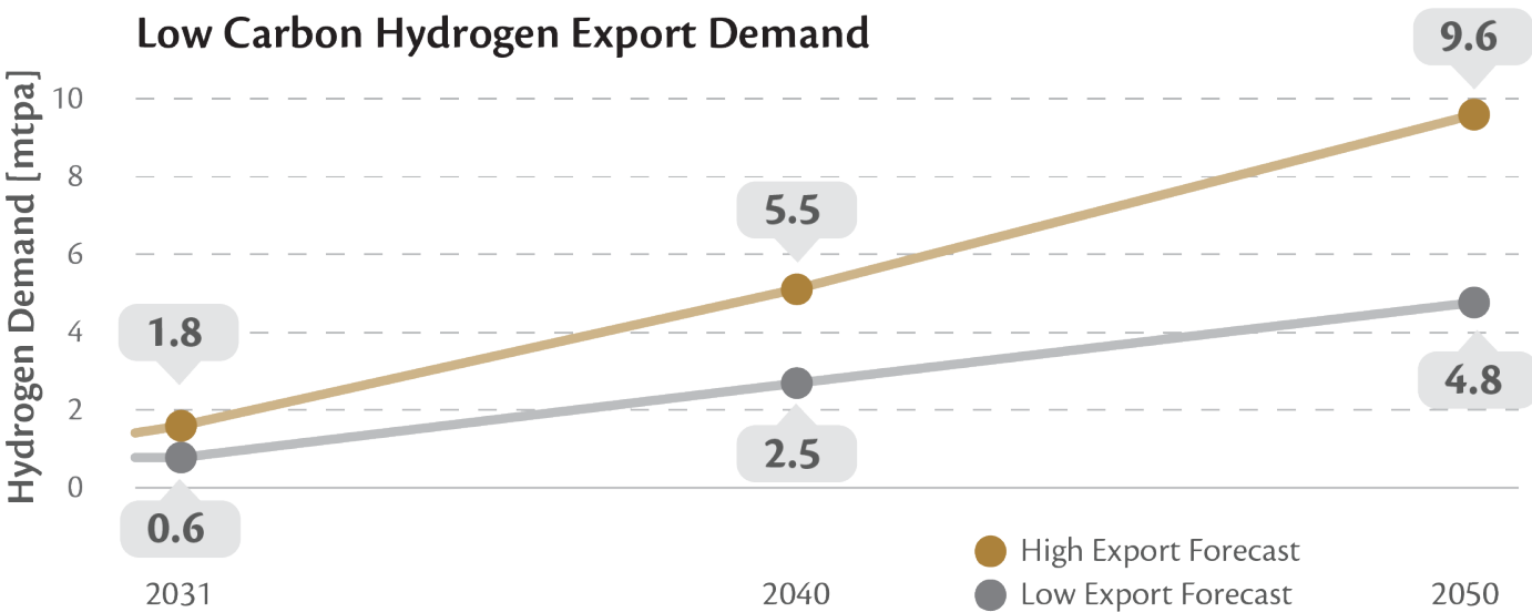
Figure 5 Low carbon hydrogen export demand (mtpa). Source: Fraunhofer CINES.
