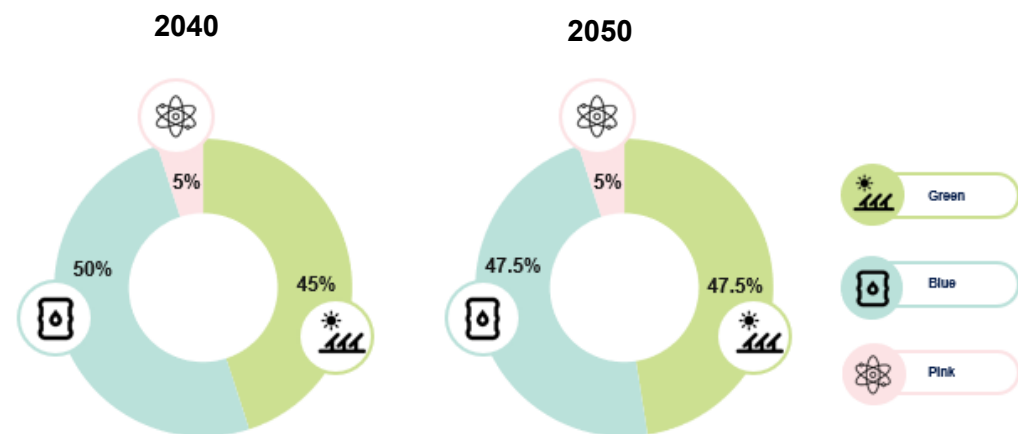
Figure 6 Shares of hydrogen colours in 2040 and 2050
