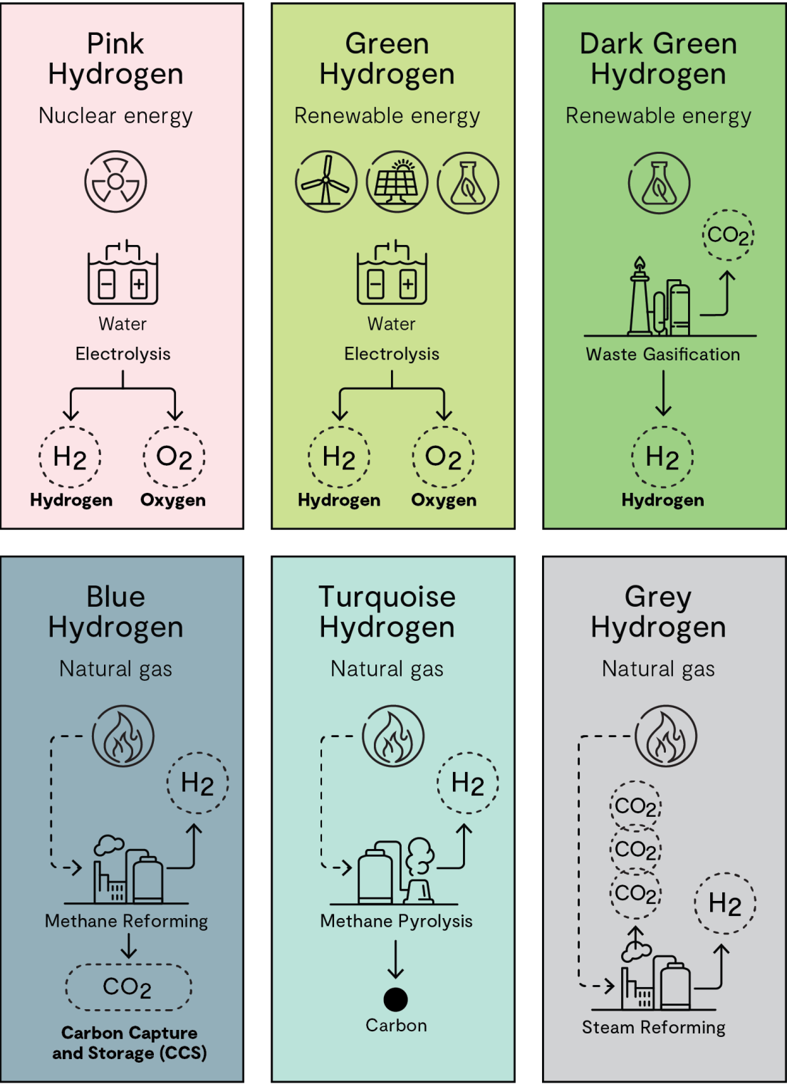
Figure 3 The different colours of hydrogen relevant to the UAE and how they are produced
