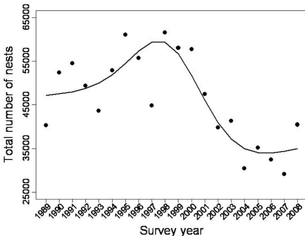
Figure 1.1.1 Annual total nest counts for loggerhead sea turtles on Florida Index beaches, 1989-2008. The trend line was estimated by fitting a five-knot restricted cubic spline curve to the total counts via negative binomial regression (FWRI 2008; Witherington et al. 2009).
